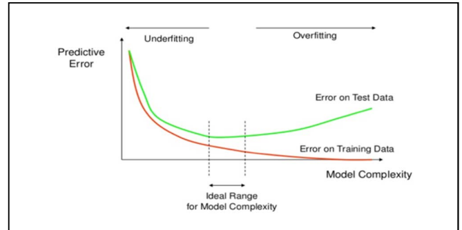
Fig. 4. Overfitting and underfitting effect on error
